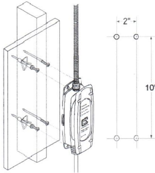
Figure 5. Mounting the LCS to a hollow wall
