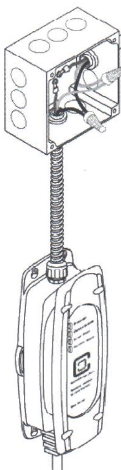
Figure 6. Wiring the LCS in a junction box
